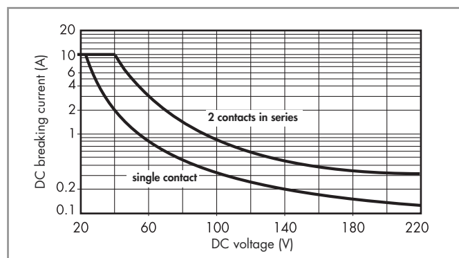
H 48 - Maximum DC1 breaking capacity Types 48.62/82
