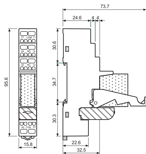
48.72 / 48.81 / 48.82 Screwless terminal
