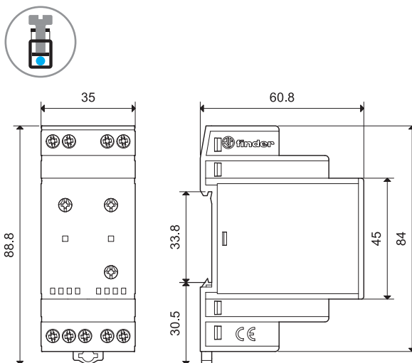
11.42 Screw terminal
