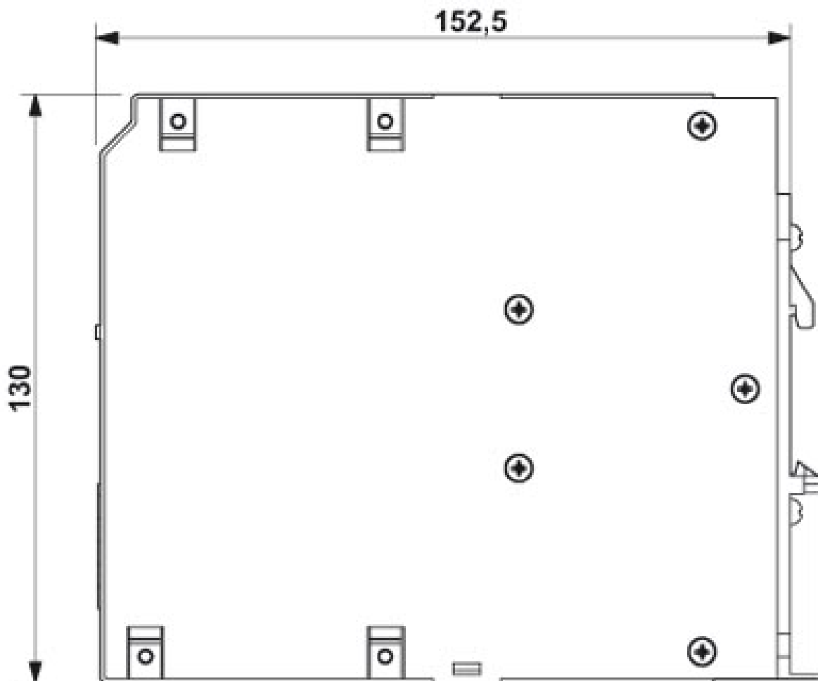
Dimensioned drawing
