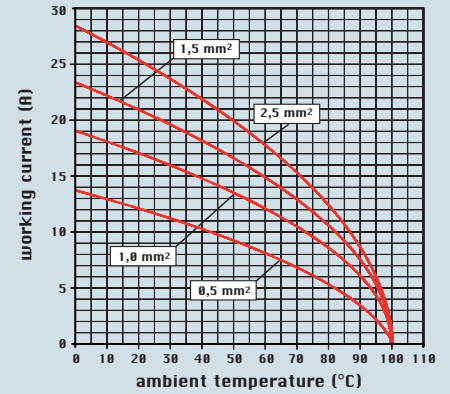
diagram CK 04 poles
