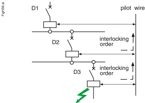
Logic selectivity
